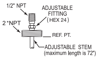
Adjustable Stem Only available with flange and 'T' type connections
